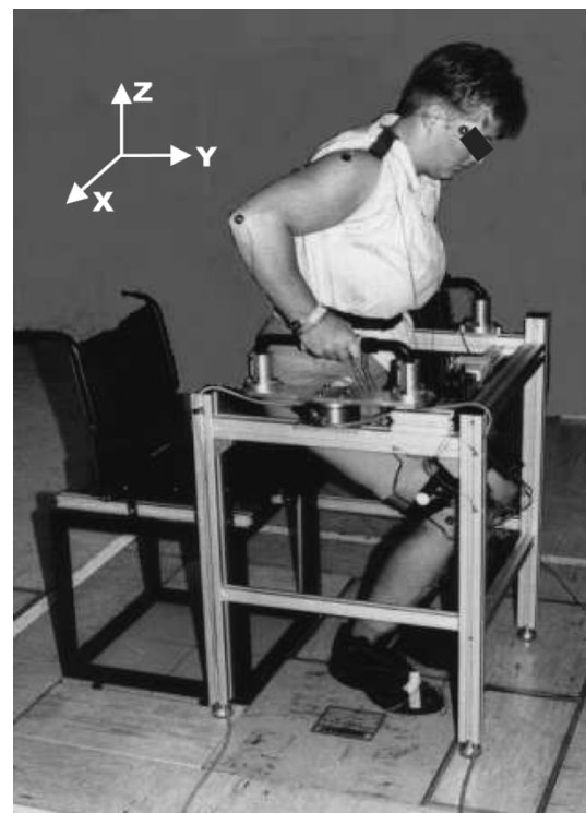
Fig. 2. Standing-up of paraplegic patient and a measurement setup.
