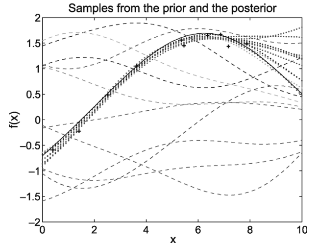
Fig. 6. Samples from the prior process (dashed lines) and from the predictive-posterior process, conditioned on the training data (crosses), for x \in [0, 10] .
