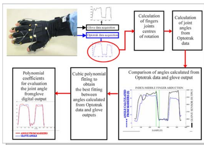
Fig 3. Data Glove calibration procedure
